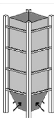
Flexible silo
